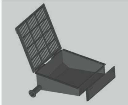
A bespoke storm overflow design for primary settlement tanks, including designs for the Copasacs, gate valves and high level alarms.
